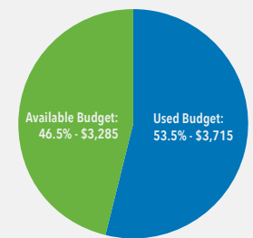
TOTAL BUDGET ($7,000)
